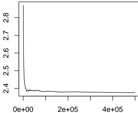
Figure 8. The log proposal standard deviation l_{s_1} corresponding to the SCAM variable \theta_1 , plotted against iteration number.
