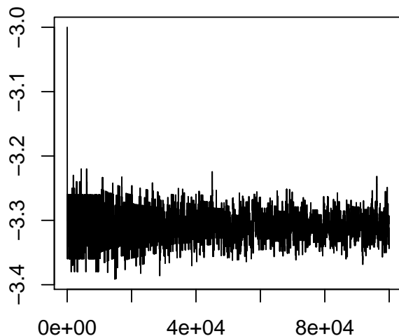
Figure 15. The tuning parameter a in the James-Stein RAMA example, plotted against batch number.
