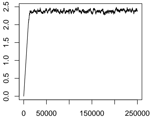
Figure 5. The log proposal standard deviation l_{s_1} corresponding to the Metropolis-within-Gibbs variable \theta_1 , plotted against batch number.
