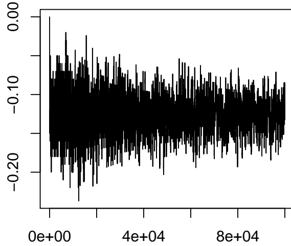
Figure 14. The tuning parameter b in the Normal RAMA example, plotted against batch number.
