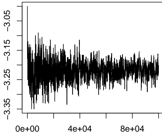
Figure 16. The tuning parameter b in the James-Stein RAMA example, plotted against batch number.
