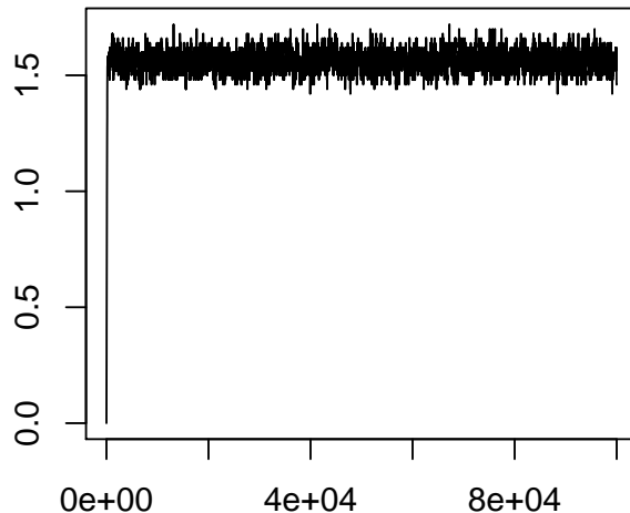
Figure 11. The tuning parameter a in the State-Dependent Scaling example, plotted against batch number, showing quick approach to “good” values near 1.5.
