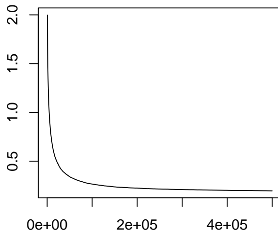
Figure 10. The log proposal standard deviation ls_3 corresponding to the SCAM variable \theta_3 , plotted against iteration number.
