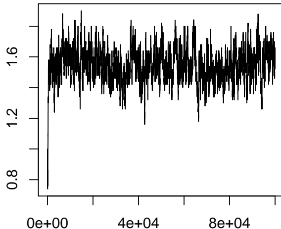
Figure 12. The tuning parameter b in the State-Dependent Scaling example, plotted against batch number, showing quick approach to “good” values near 1.6, but with significant oscillation.
