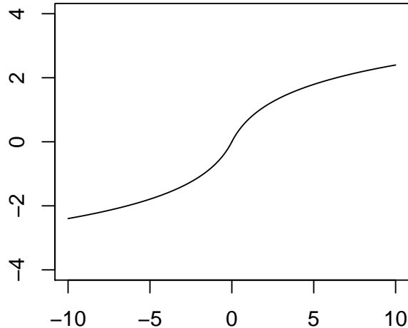
Figure 17. Graph of the modified log function \ell .
