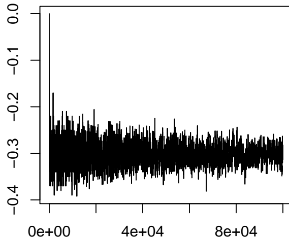
Figure 13. The tuning parameter a in the Normal RAMA example, plotted against batch number.
