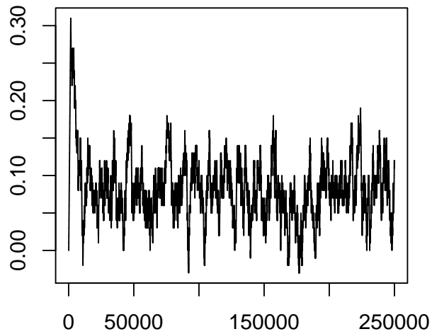
Figure 7. The log proposal standard deviation ls_3 corresponding to the Metropolis-within-Gibbs variable \theta_3 , plotted against batch number.
