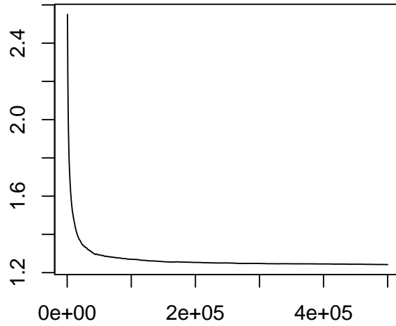
Figure 9. The log proposal standard deviation ls_2 corresponding to the SCAM variable \theta_2 , plotted against iteration number.
