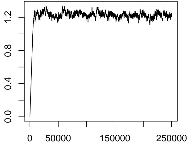
Figure 6. The log proposal standard deviation ls_2 corresponding to the Metropolis-within-Gibbs variable \theta_2 , plotted against batch number.
